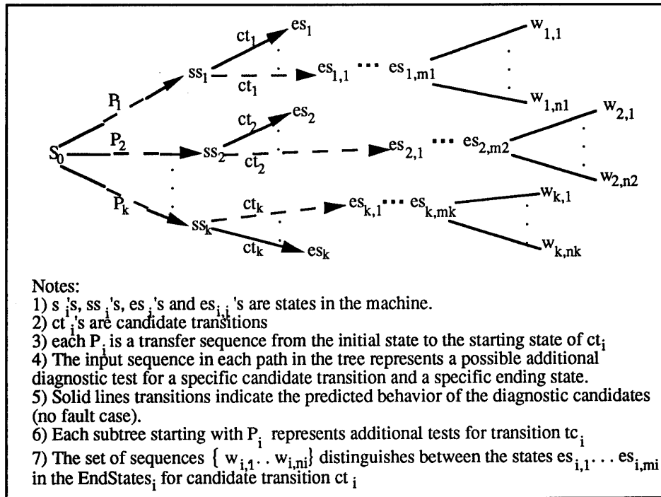
Figure 2 : Construction of additional diagnostic tests
