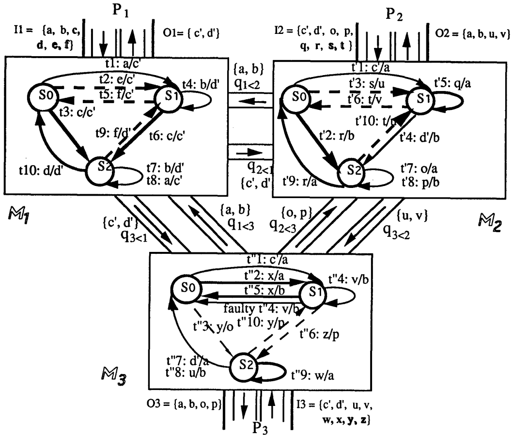
Figure 1: A state transition diagram for a three Communicating Finite State Machines
