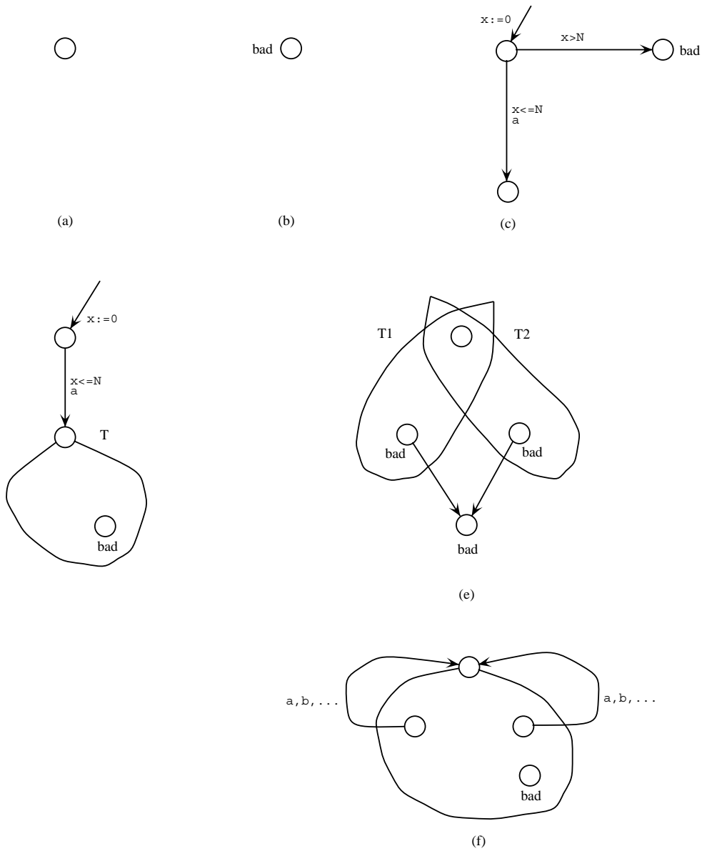
Figure 15: Generation of Testing Timed Automata: The respective test automata implements the following formulas: (a) tt , (b) ff , (c) \langle a \rangle_{\leq n} , (d) [a]_{\leq n}\varphi , (e) \varphi_1 \wedge \varphi_2 and (f) INV\varphi . In the figure, T indicates the testing automaton for \varphi . T1 and T2 indicates the automata for \varphi_1 and \varphi_2 respectively.
